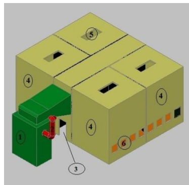
Figure 2. Technical drawing of building; 1.Burner, 2.Chimney, 3.Entrance Door, 4.Drying Rooms, 5. Loading Cover, 6. Unloading Cover
